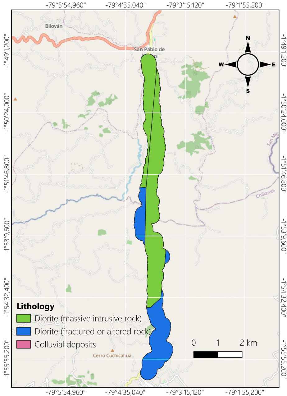
Fig. 7. Lithological map.
